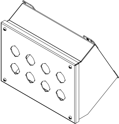
ISOMETRIC VIEW
