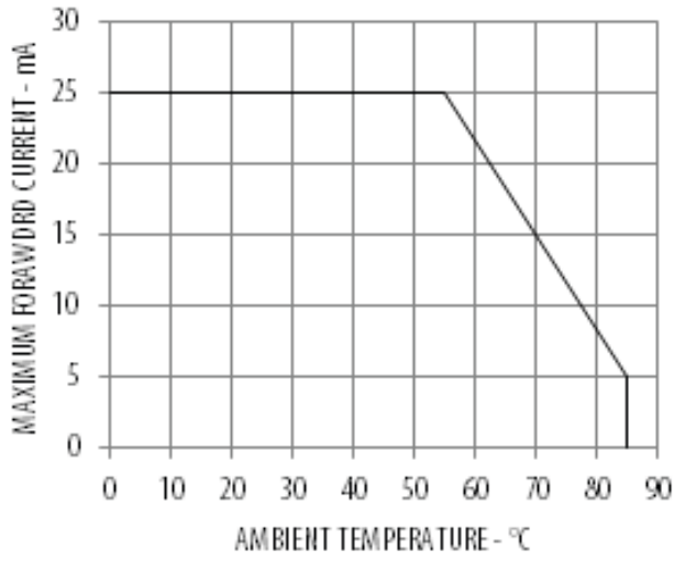
Figure 7 Derating Curve
