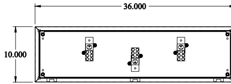
FRONT VIEW - COVER REMOVED
