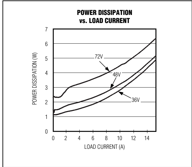
Figure 2. Power Dissipation vs. Load Current
