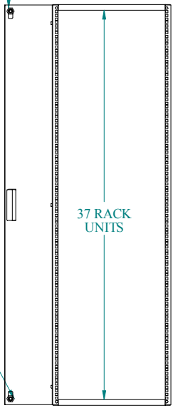
REAR VIEW
