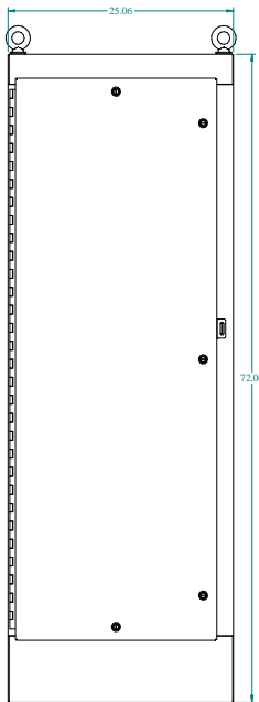
FRONT VIEW
