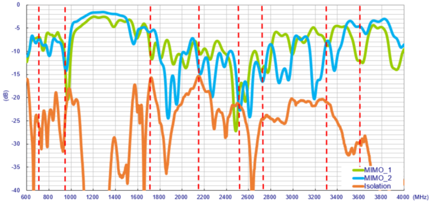
Setup on the 50*50cm ground plane with 0.3 meter cable length
