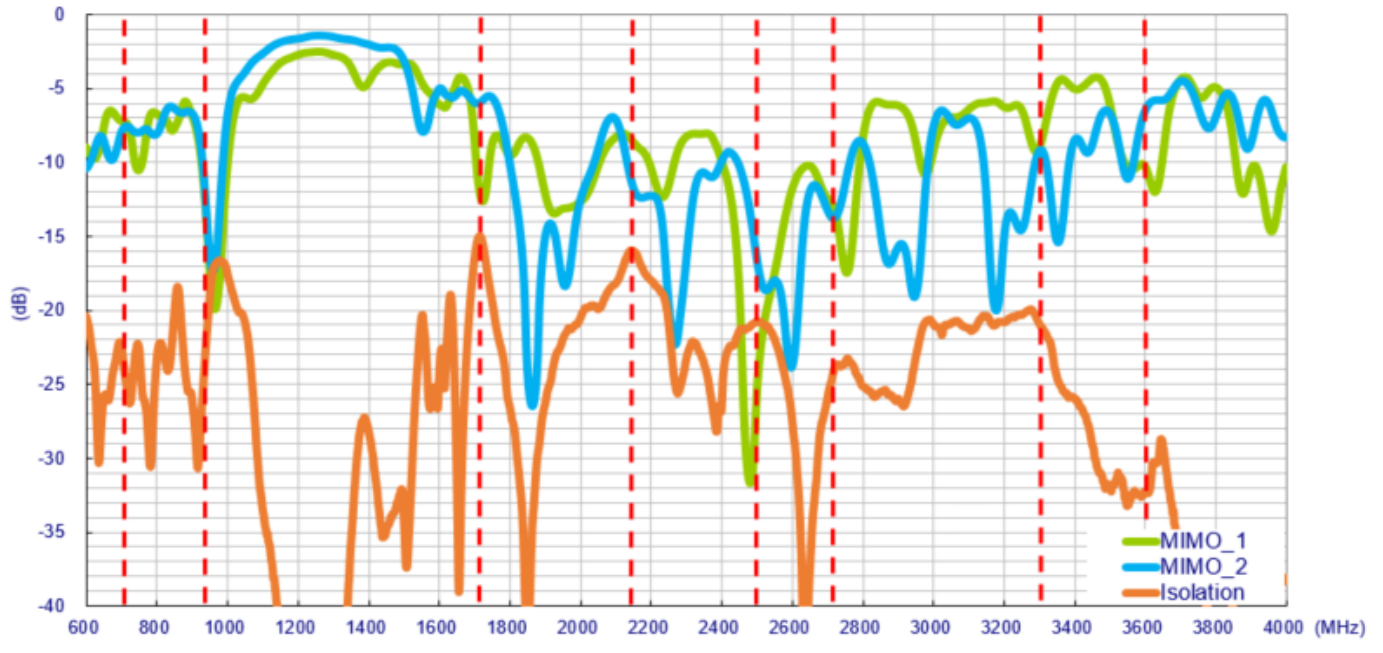
Setup in free space with 0.3 meter cable length
