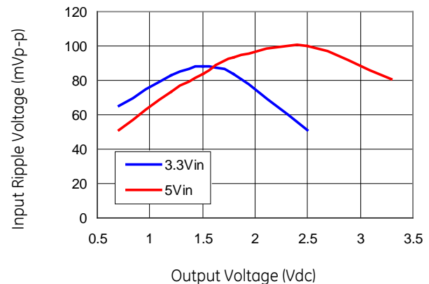
Figure 28. Input ripple voltage for various output with 3 \times 150 \mu F polymer and 2 \times 47 \mu F ceramic capacitors at the input (full load)
