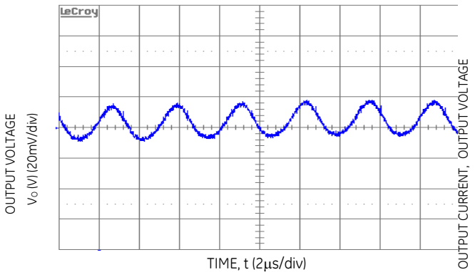
Figure 9. Typical Output Ripple and Noise (Vin = 5.0V dc, Vo = 3.3Vdc, Io=10A).
