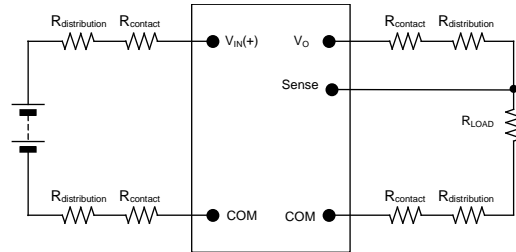
Figure 33. Remote sense circuit configuration
