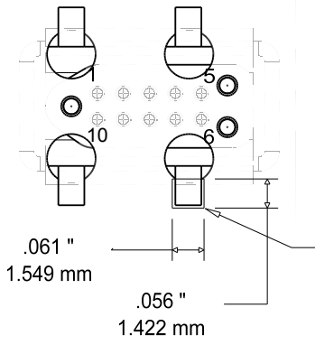
PCB BOTTOM VIEW
