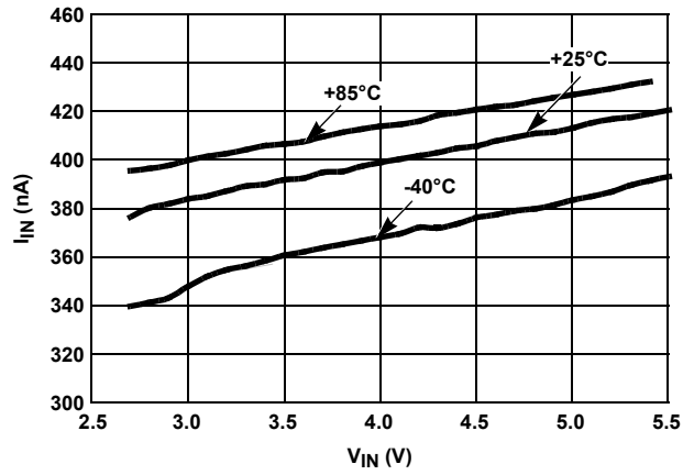
FIGURE 29. I_{IN} vs V_{IN} OVER-TEMPERATURE
