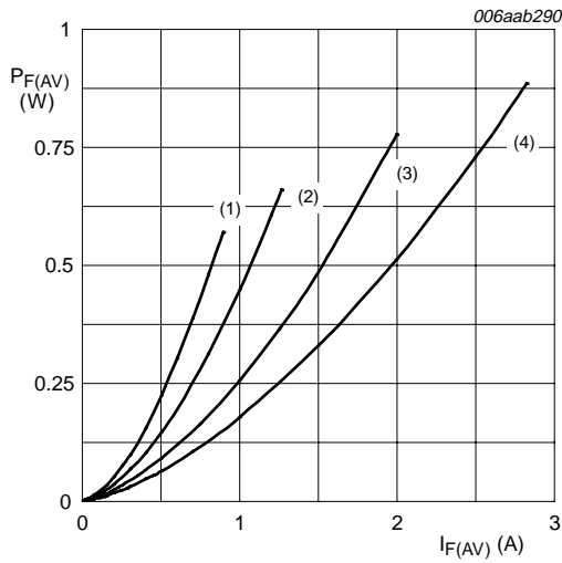
T_j = 150\text{ °C} (1) \delta = 0.1 (2) \delta = 0.2 (3) \delta = 0.5 (4) \delta = 1
