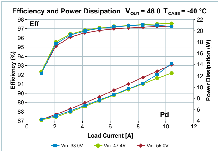
Figure 7 — Total efficiency and power dissipation vs. V IN and I OUT V OUT = 48.0 V, T CASE = -40°C
