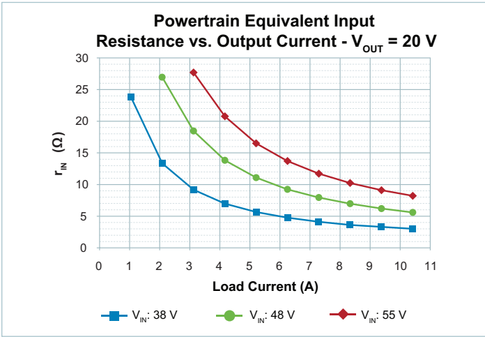
Figure 21 — Magnitude of powertrain dynamic input impedance vs. I OUT , V IN ; V OUT = 20.0 V
