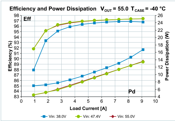
Figure 10 — Total efficiency and power dissipation vs. V IN and I OUT V OUT = 55.0 V, T CASE = -40°C
