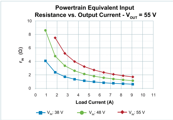
Figure 23 — Magnitude of powertrain dynamic input impedance vs. I OUT , V IN ; V OUT = 55.0 V
