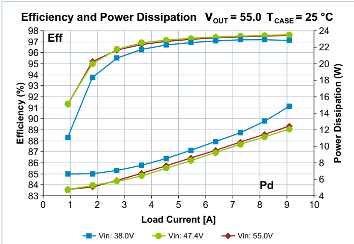
Figure 11 — Total efficiency and power dissipation vs. V IN and I OUT V OUT = 55.0 V, T CASE = 25°C
