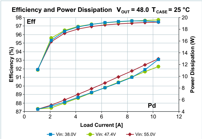
Figure 8 — Total efficiency and power dissipation vs. V IN and I OUT V OUT = 48.0 V, T CASE = 25°C
