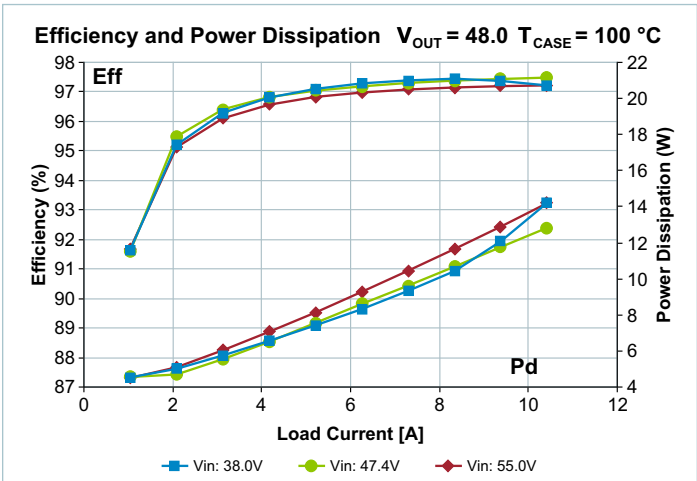
Figure 9 — Total efficiency and power dissipation vs. V IN and I OUT V OUT = 48.0 V, T CASE = 100°C
