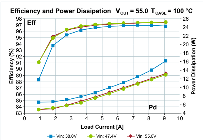
Figure 12 — Total efficiency and power dissipation vs. V IN and I OUT V OUT = 55.0 V, T CASE = 100°C
