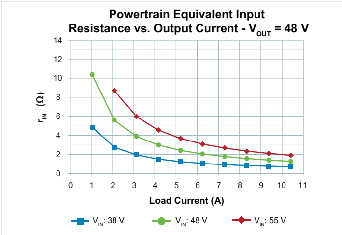
Figure 22 — Magnitude of powertrain dynamic input impedance vs. I OUT , V IN ; V OUT = 48.0 V
