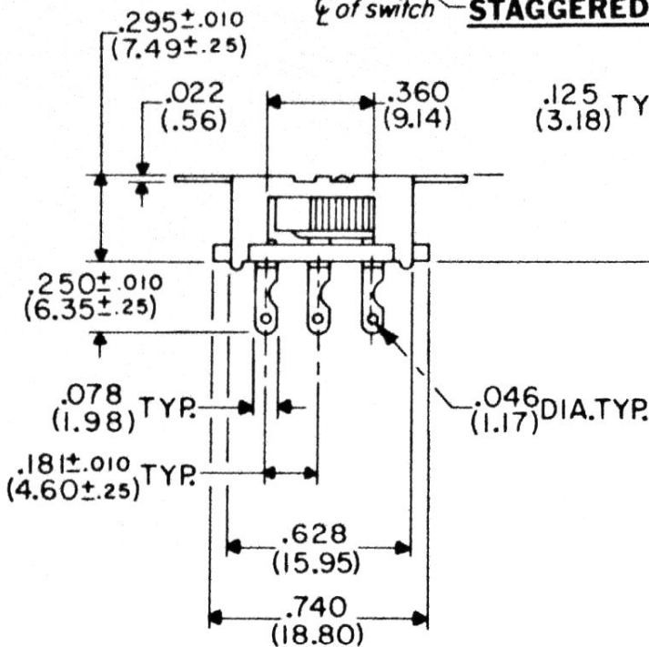
STAGGERED P.C. LAYOUT
