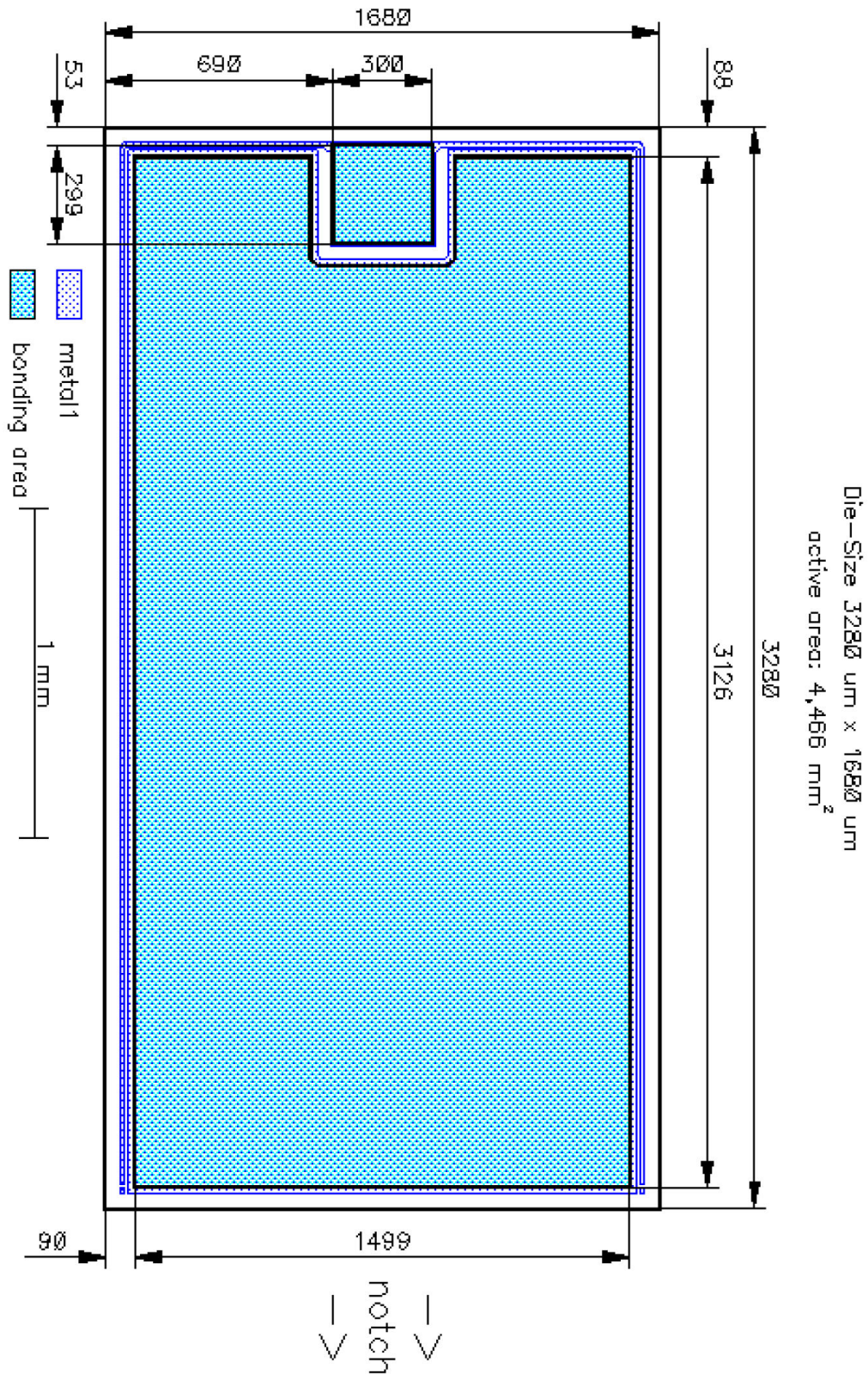
Figure 1 Outline Chip, dimensions in \mu\text{m}
