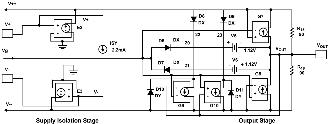
FIGURE 41. SPICE SCHEMATIC
