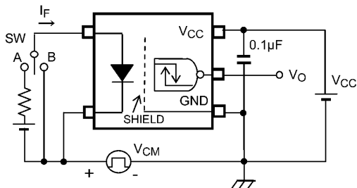
Fig. 12.1.6 Common-Mode Transient Immunity and Waveform
