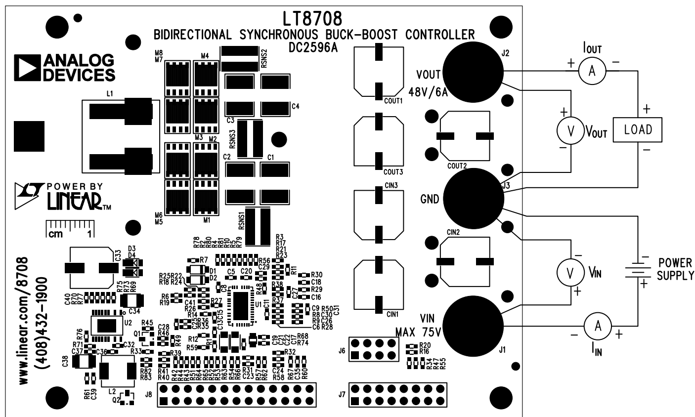
Figure 2. Test Setup
