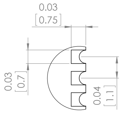
DETAIL A SCALE 10 : 1
