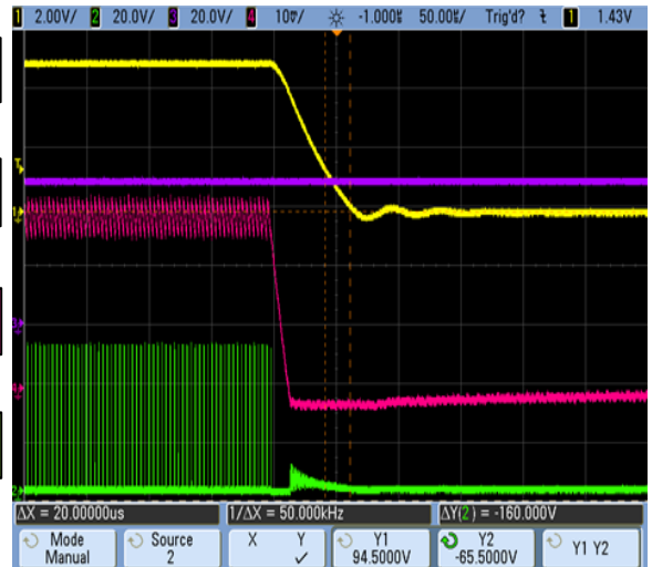
Figure 28. Shut-Down Transition at 6A Load (EN = Low)
