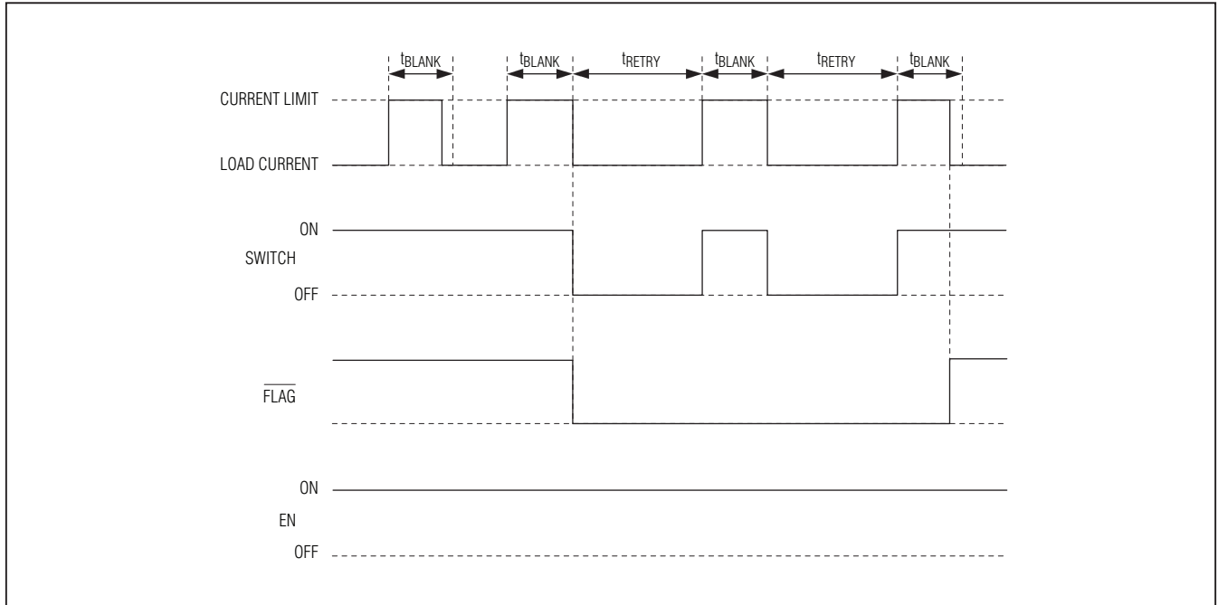
Figure 1. MAX14544 Timing Diagram (Waveforms Not to Scale)
