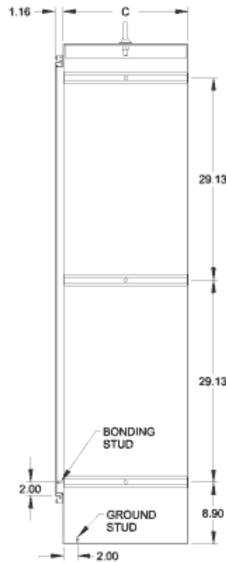
Section Y-Y
