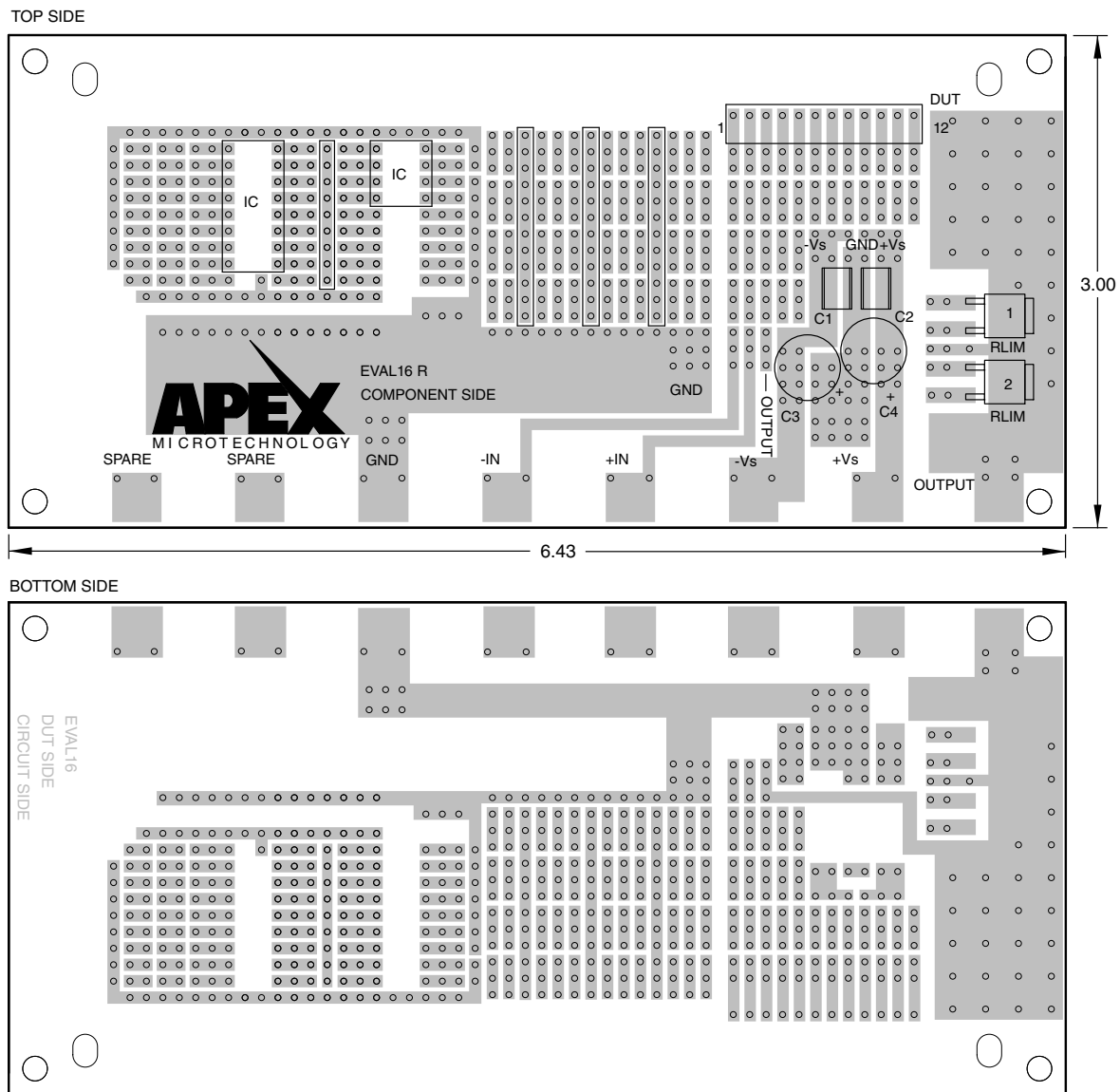
Figure 1: PCB
