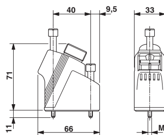
Dimensional drawing
