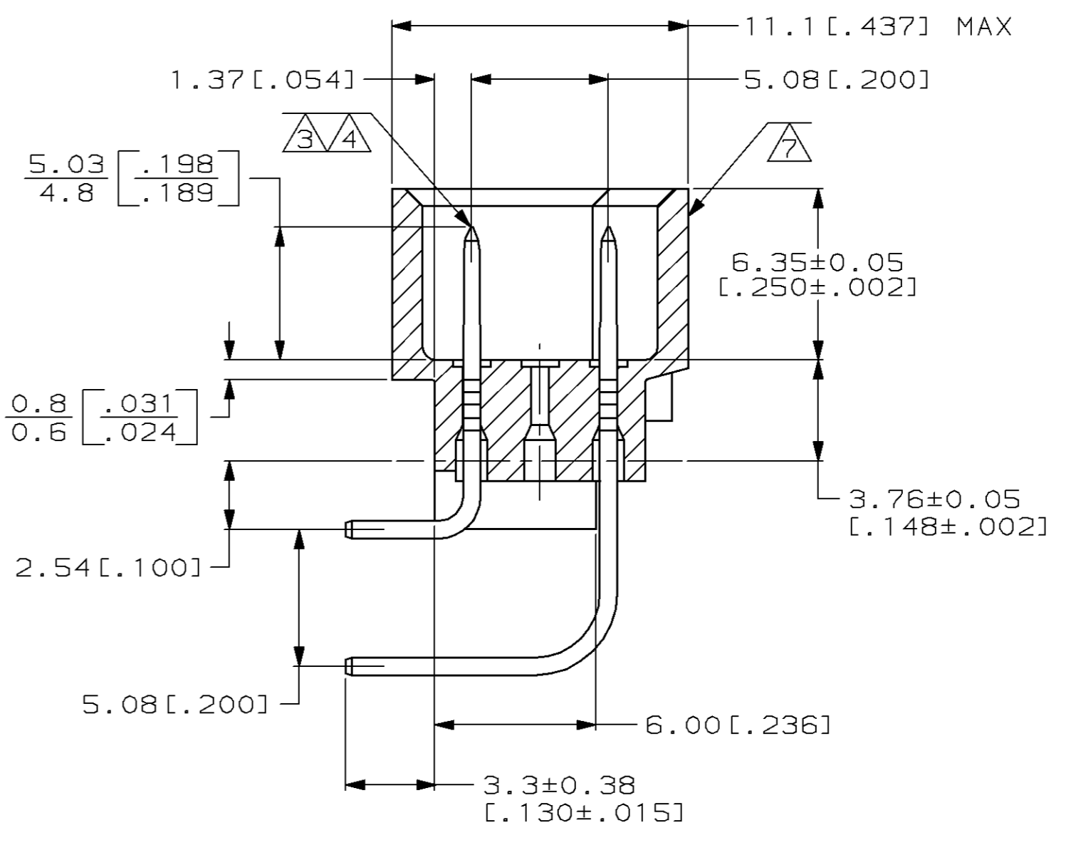
SECTION Z-Z
