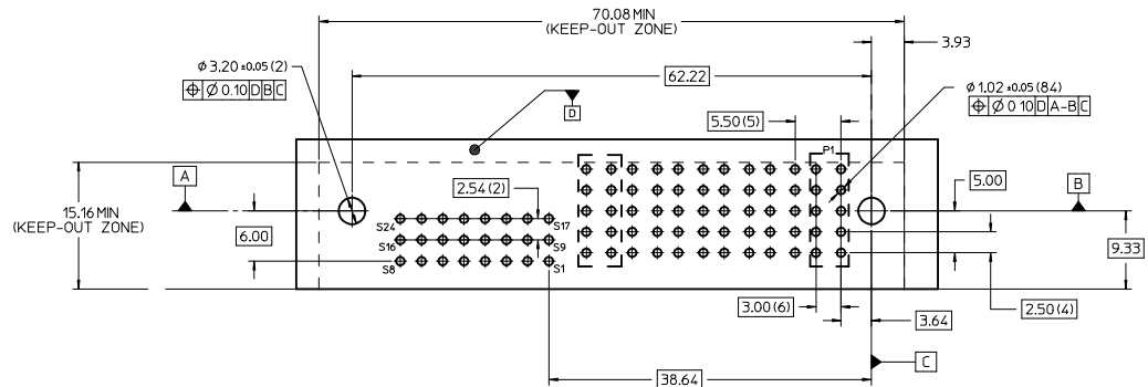
RECOMMENDED PC BOARD LAYOUT & KEEP-OUT ZONE
