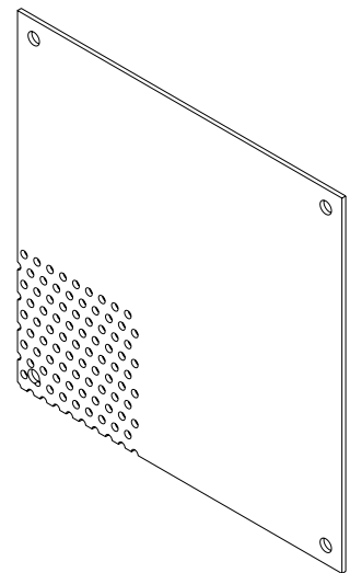
ISOMETRIC VIEW
