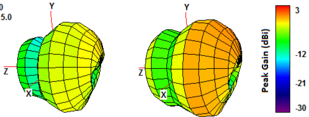
Figure 8. 3D Radiation Pattern at 1710 MHz (left), 1805 MHz (right) of the TG19 Antenna.
