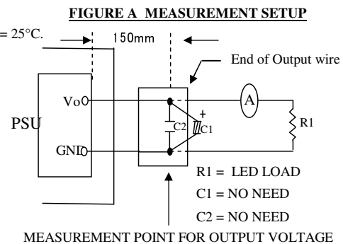
MEASUREMENT POINT FOR OUTPUT VOLTAGE
