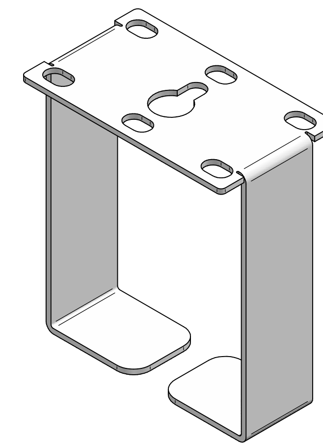
ISOMETRIC
