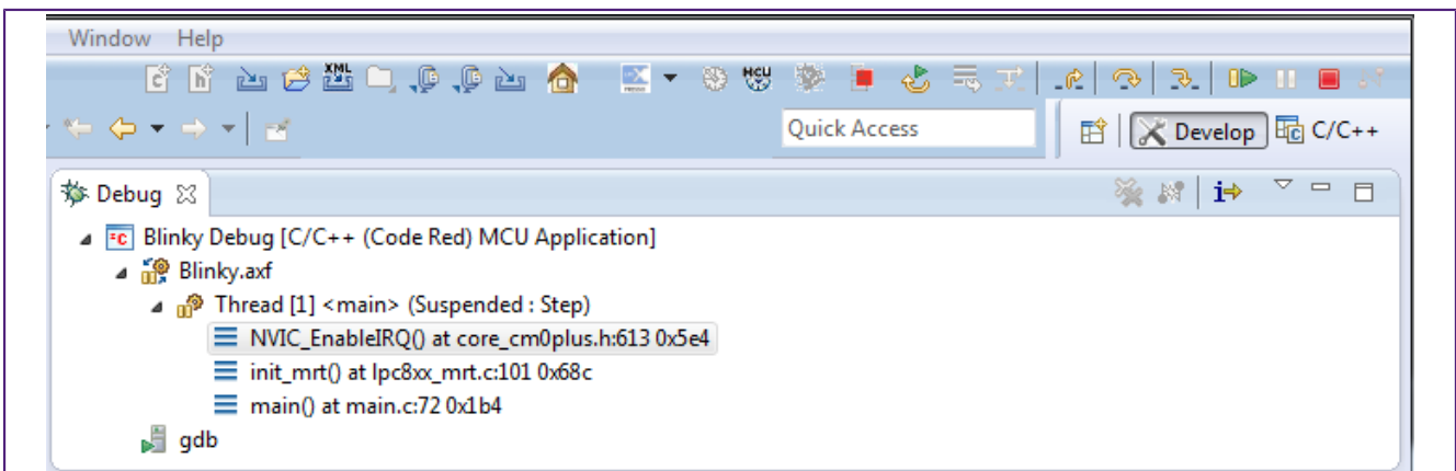
Figure 4.10. Debug Controls
