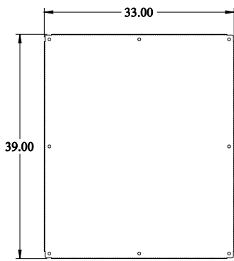
INNER PANEL
