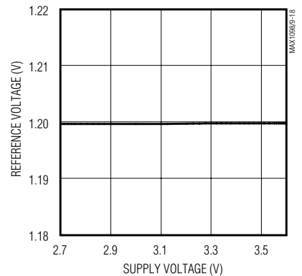
MAX1099 INTERNAL REFERENCE VOLTAGE vs. SUPPLY VOLTAGE
