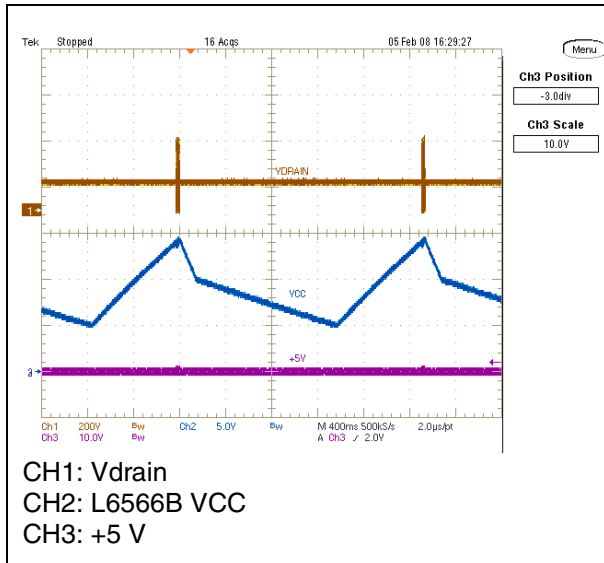
Figure 24. EVL6566B-40WSTB output short +3.3 V at 90 V - full load
