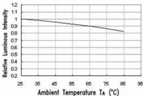
Ambient Temperature T_a (°C) Fig.5 Luminous Intensity vs. Ambient Temperature
