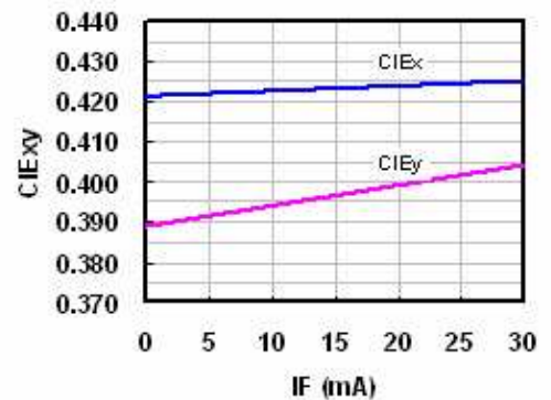
Fig.7. CIE xy vs. Forward Current
