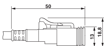
Dimensional drawing
