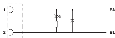
Contact assignment of the DEUTSCH DT06-2S
