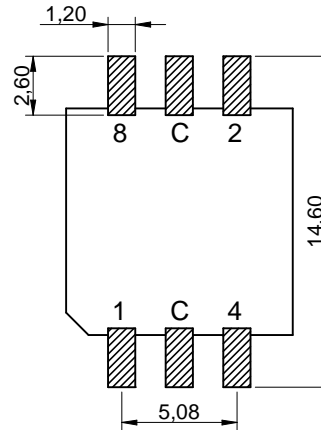
RECOMMENDED LAYOUT
