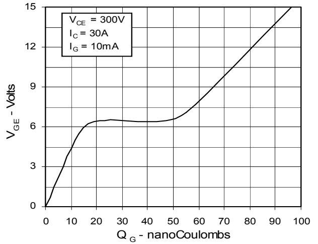
Fig. 14. Gate Charge
