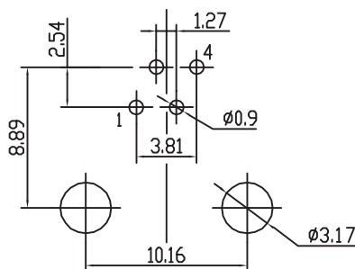
PCB LAYOUT - COMPONENT VIEW
