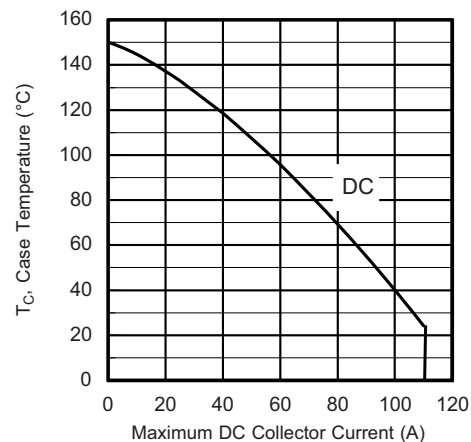
Fig. 6 - Maximum Collector Current vs. Case Temperature
