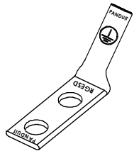
TWO HOLE ESD PORT BENT 45° (QTY. 1)
