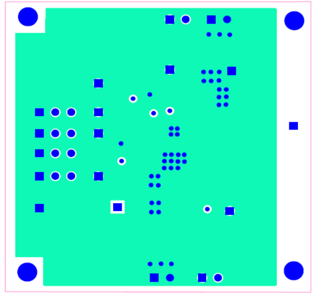
Figure 18. 2 nd Layer
