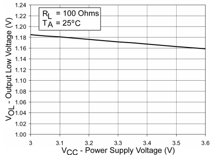
FIGURE 10. Output Low Voltage vs. Power Supply Voltage
